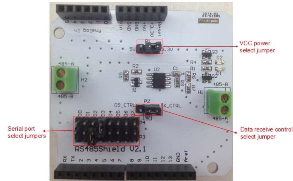
title=File:RS485_v2_jumpers.jpg)
